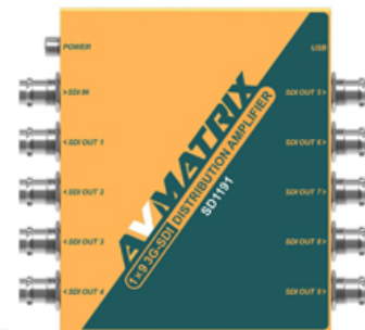
3G-SDI 1x9 Reclocking Distribution Amplifier
